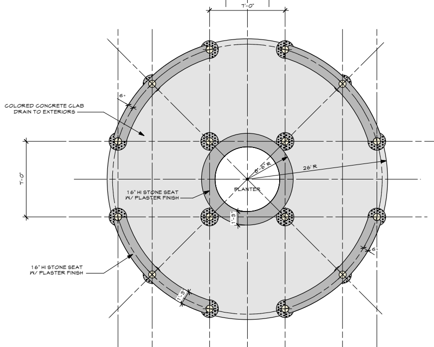
PLAN 'A' FOUNDATION
